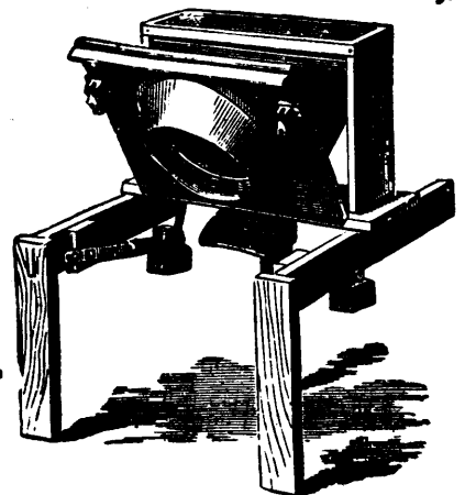
Self-Acting Apparatus.
