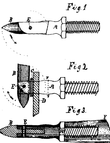
35589 Cox's Safety Whiffletree Trace Fastening.
