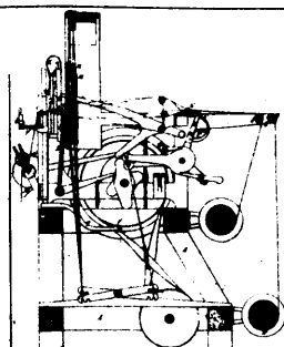
5916 Chapman's Improvements on Looms for Weaving Suspender, &c.
