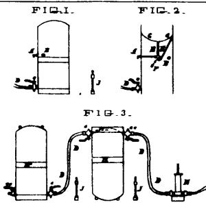
5907 Murphy, Taylor & Hayward's Pneumatic Fire Extinguisher.
