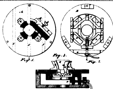
5908 Newcomb's Treennail Machine.
