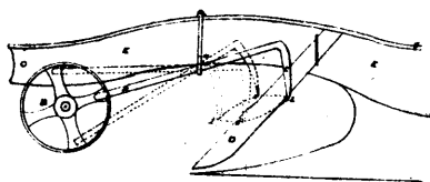
4983 Moore's Machine for Cleaning Ploughs.
