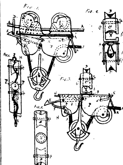
21020 Hall, Robinson & Beane's Hay-Carrier Machine.
