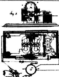
No. 1885. Hoovenbergh's Printing Telegraph.
