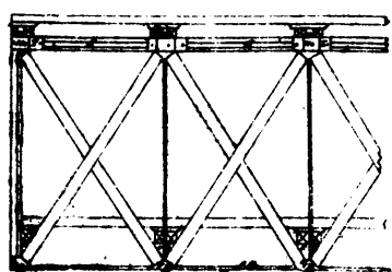
No. 1886. Anderson's Formation of Spans of Bridges.
