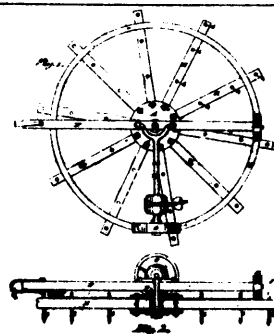
No. 1877. Burdick's Rotary Harrow.
