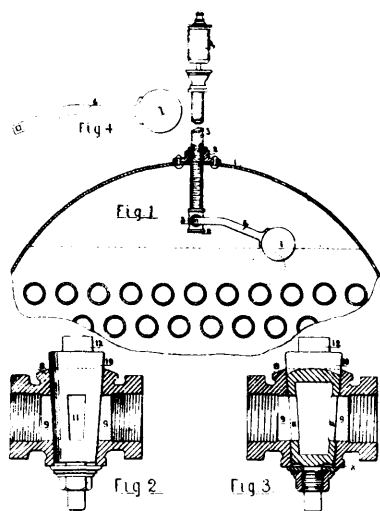
36807 Hampton and Holden's Low Water Alarm Whistle.
