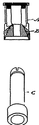
29756 Malcolm's Water Cock
