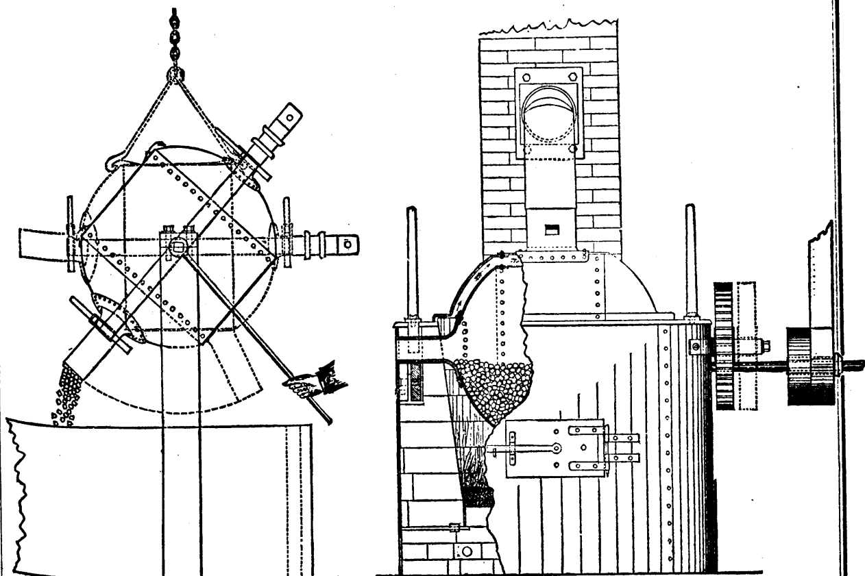
THE GILL ANNEALING FURNACE.
