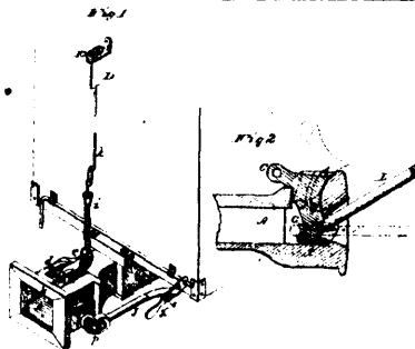
6393 Perry's Improvements on Car-Couplings.
