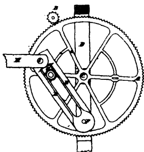
3/92 Smallwood's Lever Feed for Shingle Sawing Machines.
