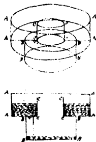
3300 Pearson &amp; McLane's Steam Generator.
