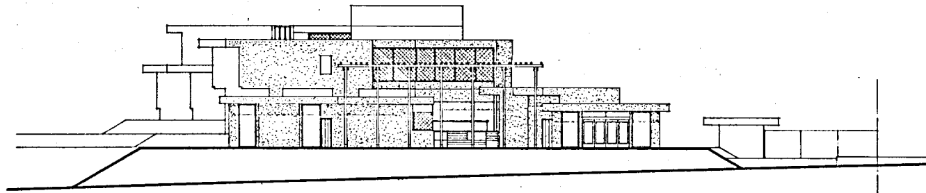
EAST ELEVATION
