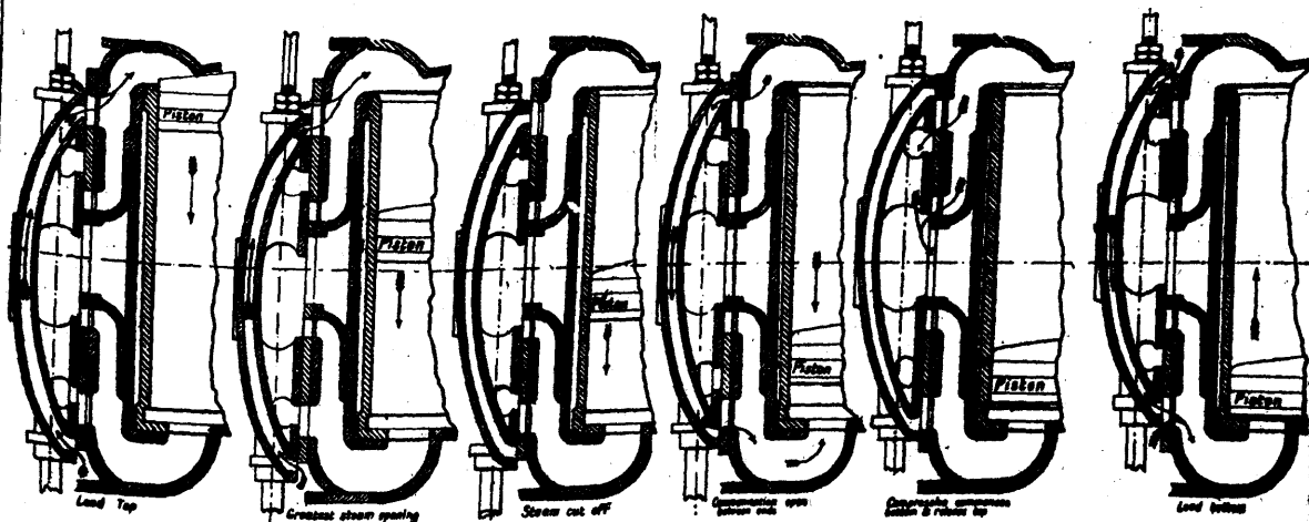
THOM'S SLIDE VALVE.
