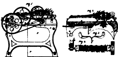
4704 Moulton &amp; Thompson's Bark Rasping Machine.
