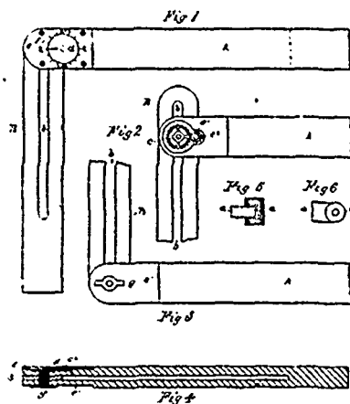
24533 Friess &amp; Todd's Bevel.
