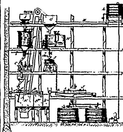
24534 Schuman's Manufacture of Starch.
