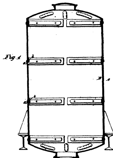
21486 Ritter &amp; Killner's Apparatus for the Manufacture of Cellulose, &amp;c.
