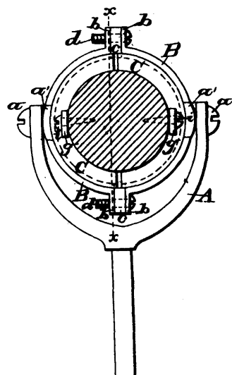
21489 Marshall's Bow Lock.
