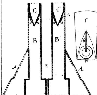
20303 Pickard &amp; McDonald's Washing Machine.
