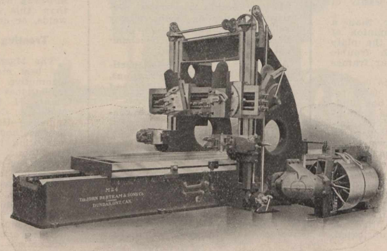
54-inch x 54 inch Iron Planing Machine with Patented Four-Belt Drive
