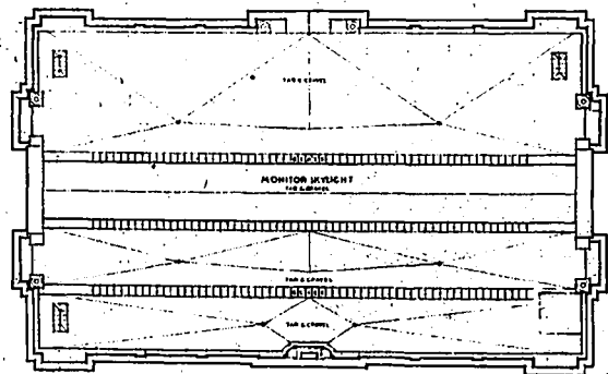
ROOF PLAN
