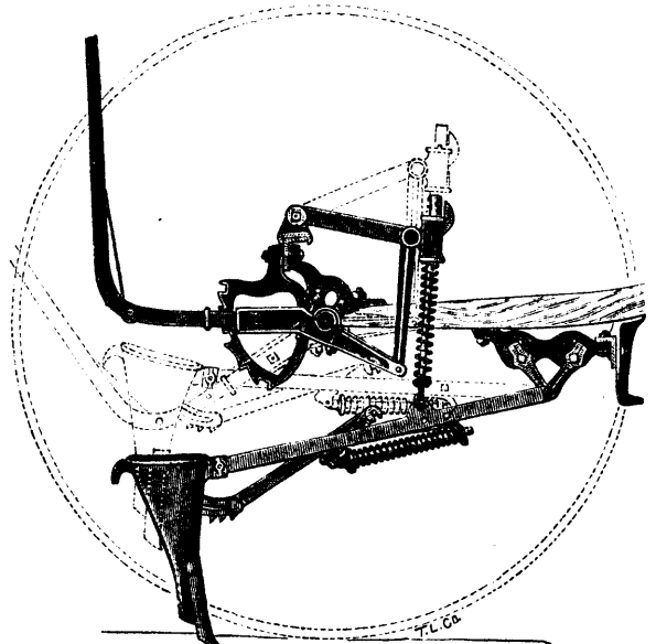
JUST ONE LEVER APPLIES THE PRESSURE, OR, REVERSED, LIFTS THE HOES FOR TRANSPORTATION—SIMPLY PERFECT. THE DOTTED LINES SHOW THE OPERATION. SUCH IS ONE OF MANY SUPERIOR POINTS ON THE MASSEY-HARRIS COMBINED HOE DRILL AND BROADCAST SEEDER.
