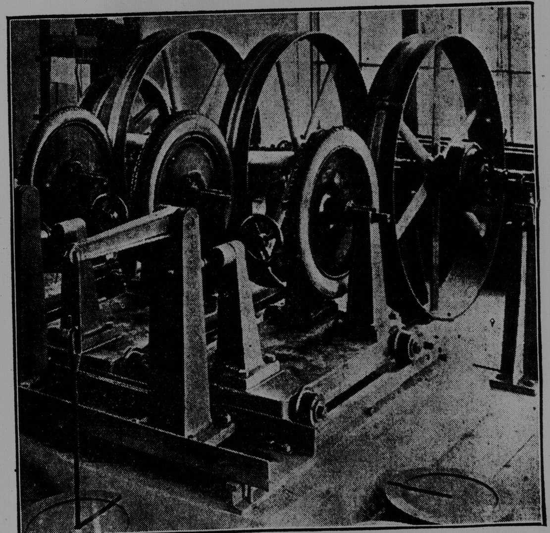
HOW LONG WILL TIRES LAST?—Testing Them Out in Washington, With Pressure Against Wheels, With Road-like Surface, Bumps and All. They Are Run Day and Night Until Worn Out.
