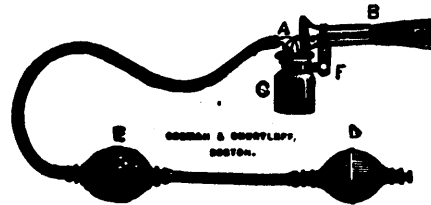
Shurtleff's Atomizing Apparatus. Pat. March 24, 1888.
