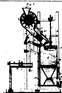
11264 Stoner's Improvements on Weighing Machines.
