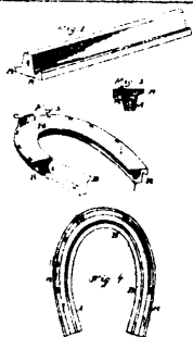
11265 Billings's Improvements on Horseshoes.
