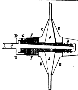
11260 Newman's Improvements on Metallic Hubs.
