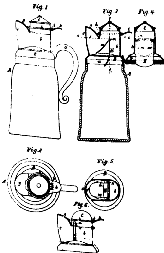
34581 Hazelton's Vessel for Measuring Sugar, etc.
