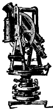
DAVIS'S IMPROVED HEDLEY DIAL
