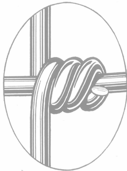
"AMERICAN" Fence Knot
