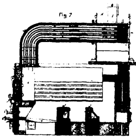
10298 Marland's Method of Utilizing the Heat of Boiler Furnaces.
