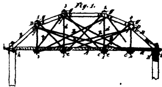
10295 Jarvis' Improvements in Bridges.
