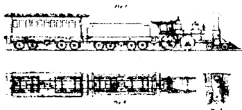
2068 Gardner's Steam and Air Car-Brakes.
