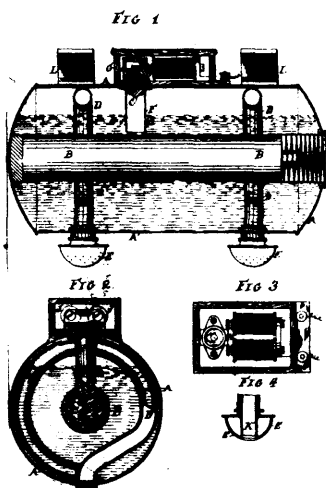
30866 Douse's Electrically Controlled Apparatus for Preventing Fires, etc.
