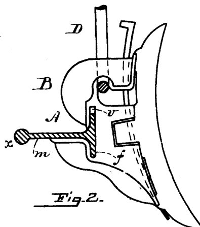
30866 Douse's Electrically Controlled Apparatus for Preventing Fires, etc.
