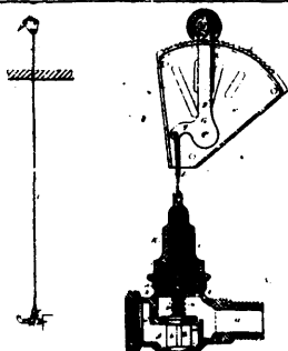
3692 Seal's Gas Cut off and Regulating Cock.
