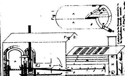
3690 Wright's Drying-house.
