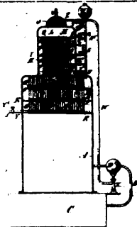
3687 Ruthven's Gas Machine.
