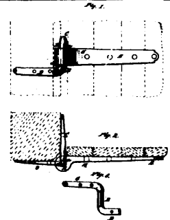
3691 Doane & Harris's Improvements on Hinges.
