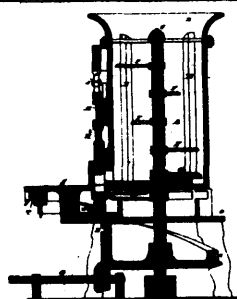
3693 Macaulay's Brick-Machine.
