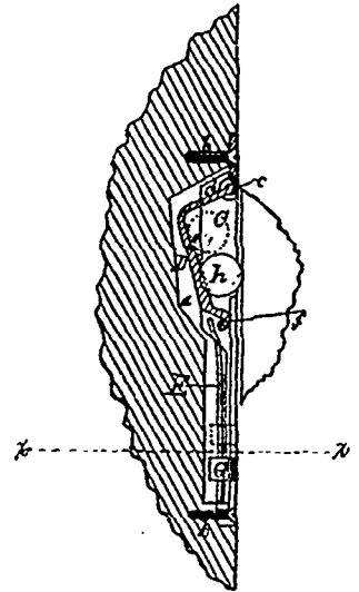
23715 Byam's Sash Balance.
