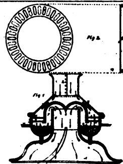
7735 June &amp; French's Spark Arrester.
