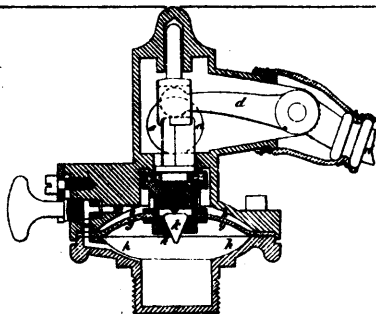
7730 Jennings's Improvements on Sinks and Water-Closets.
