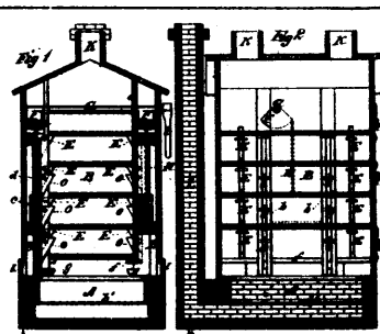
7726 Craven's Improvements on a Drying House.
