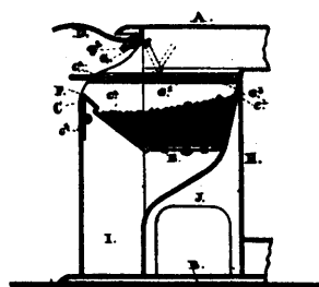
7727 Hamlin's Improvements in Cooking and Heating Stoves.
