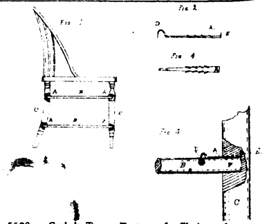
5589 Craig's Tenon Fastener for Chairs and other Furniture.
