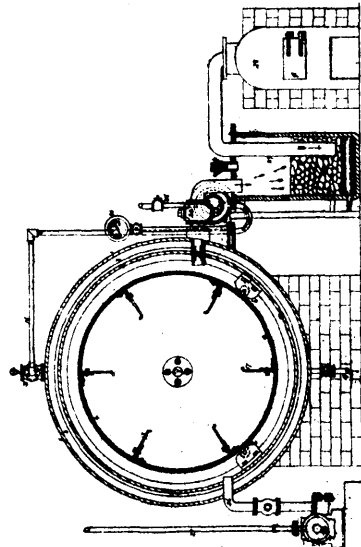
20828 Illingworth's Method of, and Apparatus for Treating Fibres, &c.
