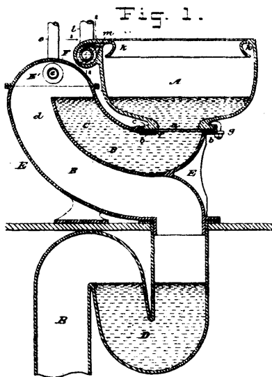
20824 Boyle's Pipe Connection for Water Closet Bowls, &c.
