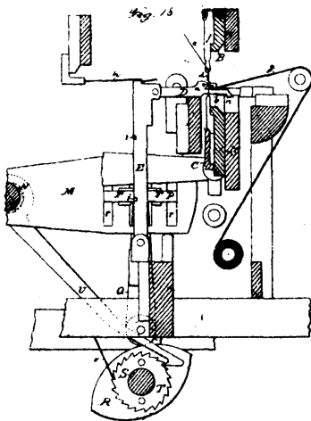
20827 Chapman's Knitting Machine.
