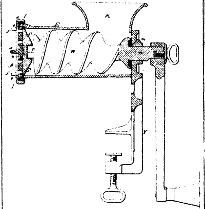
20826 Baker's Meat Cutter.
