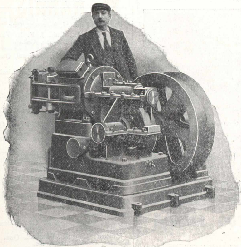
Winch Worm Drive—One Ton at 80 feet per minute—Series Motor with Flapper Brake
