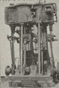
15 AND 30-20 HORSE AND AFT. COMPOUND MARINE ENGINE WITH STEAM REVERSE
