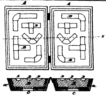
2896 Parker's Improvements on the Art or Process and Mould for Casting Cores.
