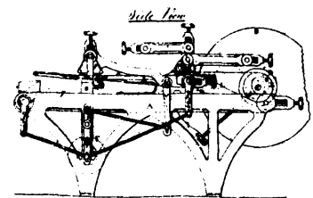
2909 Copping's Improvements on Lozenge Machines.
