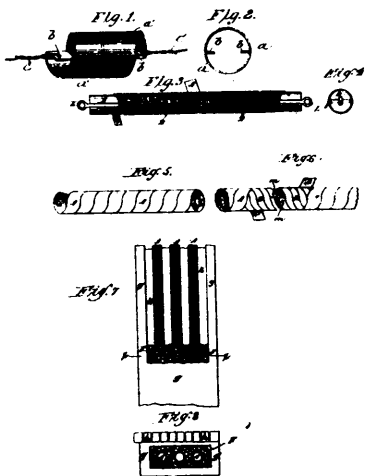
37408 Chenoweth's Method of and Apparatus for Moulding the Inner Surfaces of Vessels, etc.
