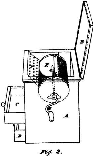
37416 Flack and Elliott's Machine for Sifting Coal.
