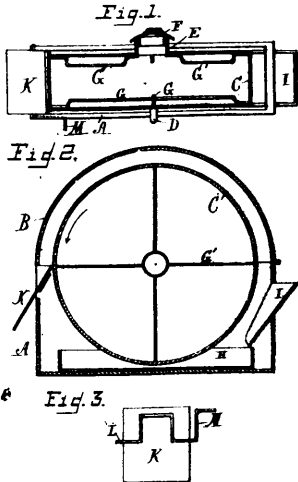
37411 Camp's Machine for Cooling and Purifying Liquids.
