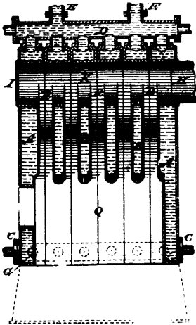
37407 Howatt's Sectional Water Heater.
