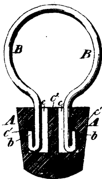
28099 Noble's Electric Arc Lamp.
