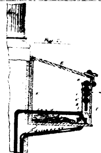
2713 Haxton & Shurtleff's Machine for Stamping Letters and Obliterating Stamps.
