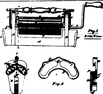
7037 Calkins' Improvements on Washing Machines.
