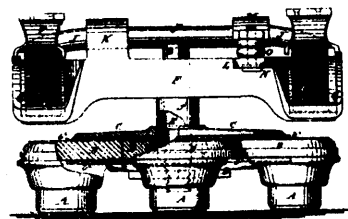
4345 Doremus' Oscillating Spring Chair.
