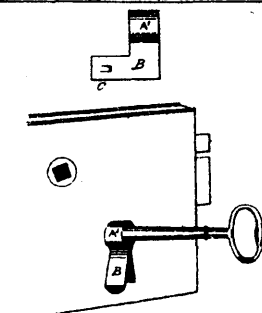
4330 Kinney's Lock and Key Guard.
