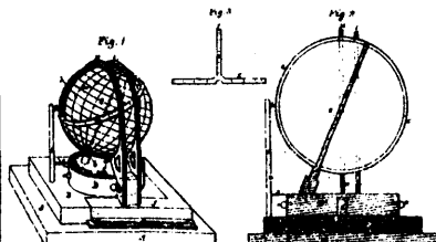
4344 Fitz's Method of Mounting and Operating Globes.
