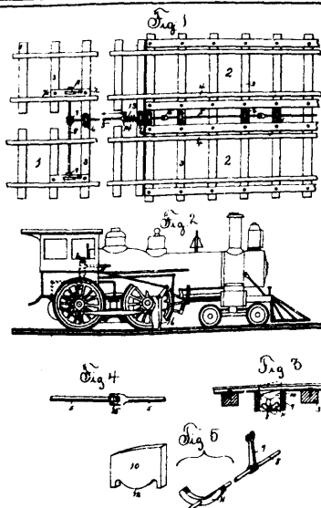
35655 Graff's Railway Appliances.
