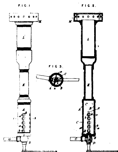
Cox's Gas Burner.
