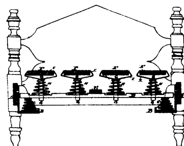
2036 Watt's Spring Bed Bottom.
