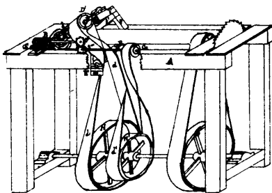
2025 Butler &amp; Duclos's Machine for Cutting Laths.
