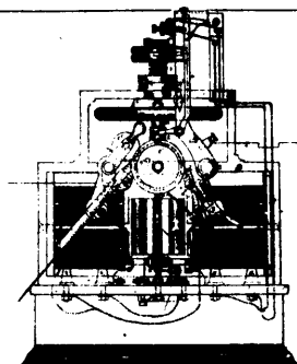
2039 Little's Electric Telegraph Apparatus and Circuit.
