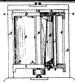
2027 Dodson's Grain Scourer.
