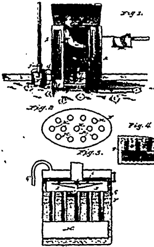
25055 Douglass's Vapour Generator.
