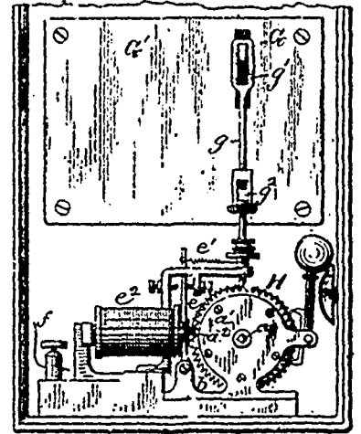
25067 Rogers's Fire Alarm Apparatus.
