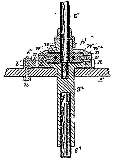
25070 Willson's Clutching Mechanism for Car Brakes.
