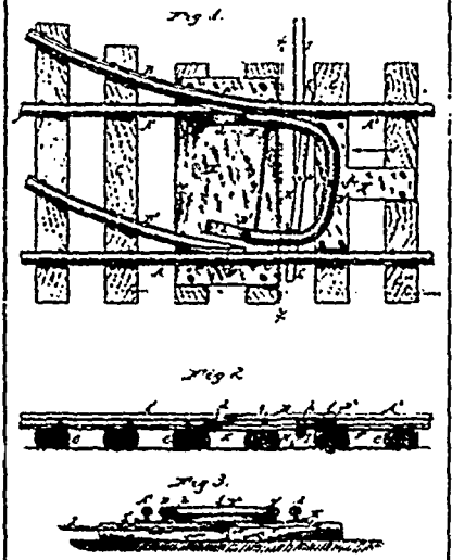
25073 Batt's Railway Switch.
