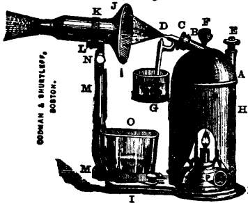
Fig. 1. The complete Steam Atomizer.
