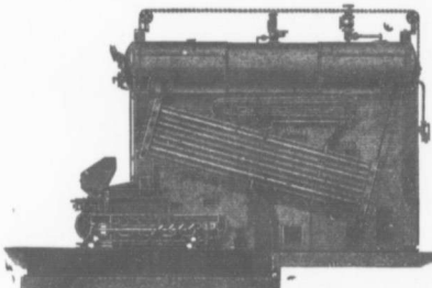
"B. & W." PATENT WATER TUBE BOILER. SUPERHEATED AND IMPROVED MECHANICAL STOKER.
