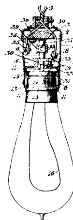
38539 Bryant's Incandescent Lamp Socket.
