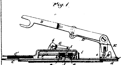
13378 Harris's Improvements on Sewing Machines.
