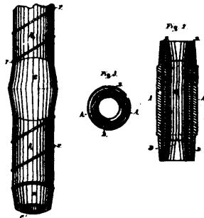
13386 Moulton's Improvements on Water Tubing.
