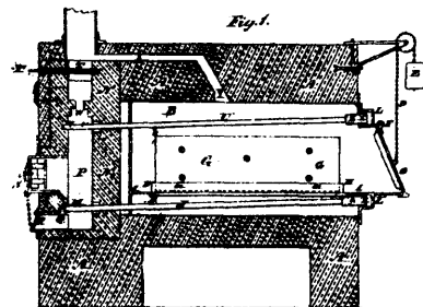
13379 Henley's Improvements on the Process of Treating Dates, and Apparatus Therefor.
