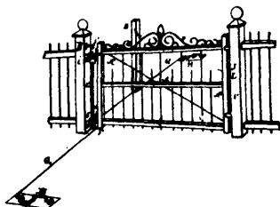
13390 Long's Improvements on Swinging Gates.
